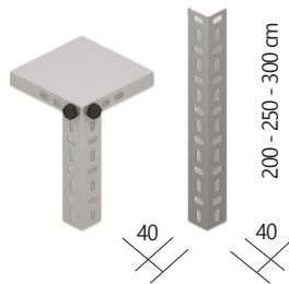
Çelik Raf Profil (40x40) Steel Shelf L Profile (40x40)
