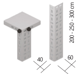
Çelik Raf Profil (40x60) Steel Shelf L Profile (40x60)
